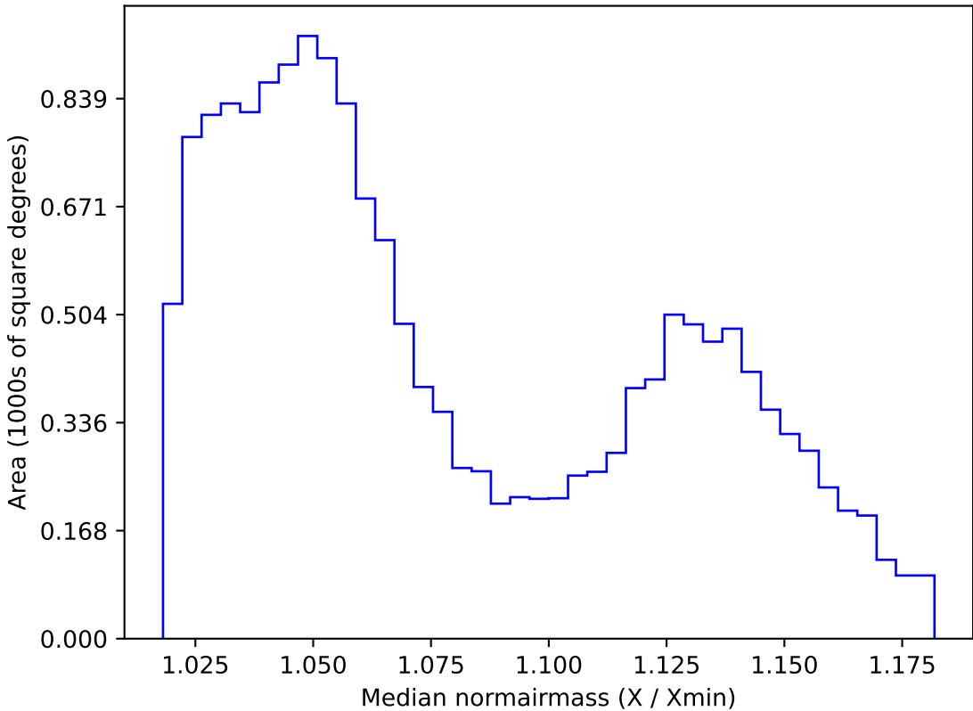
too_combined_s0.5_v3.4_10yrs WFD r band: Median normairmass
