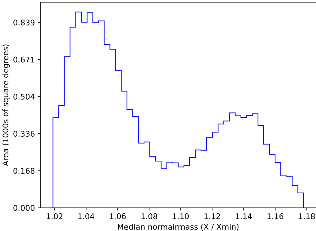
too_combined_s0.5_v3.4_10yrs WFD i band: Median normairmass
