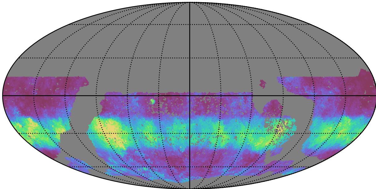
too_combined_s0.5_v3.4_10yrs WFD g band: Median normairmass
