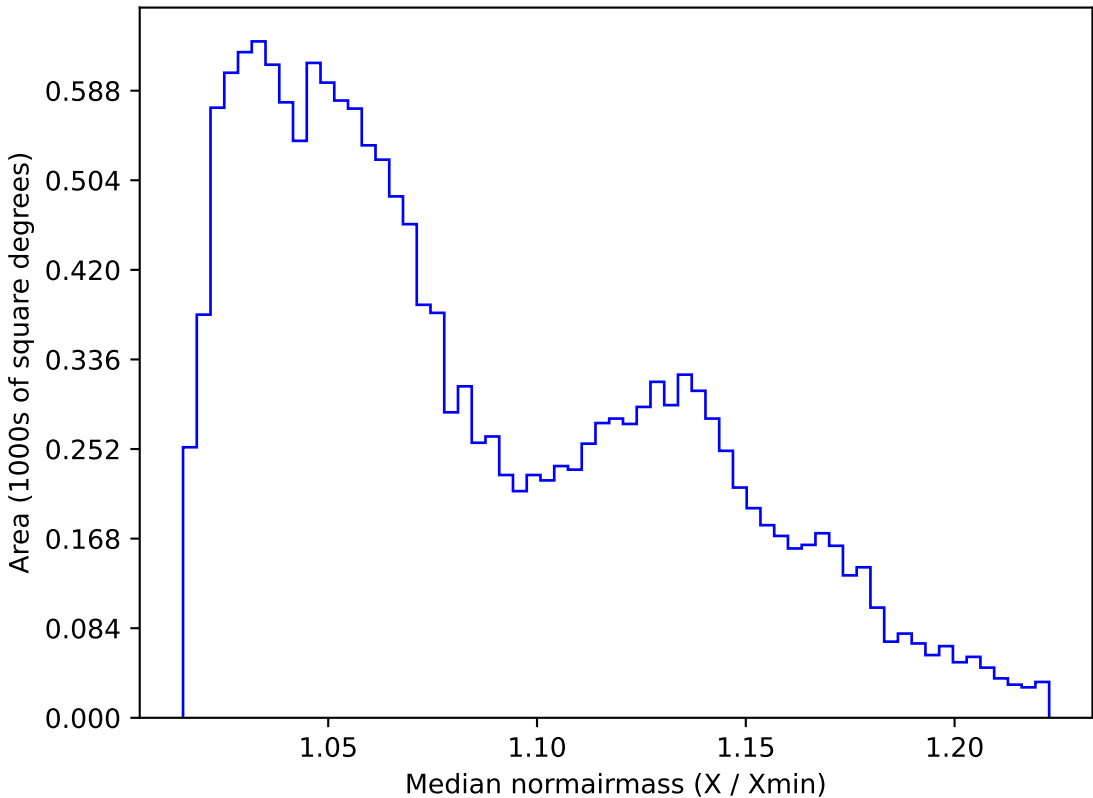
too_combined_s0.5_v3.4_10yrs WFD g band: Median normairmass
