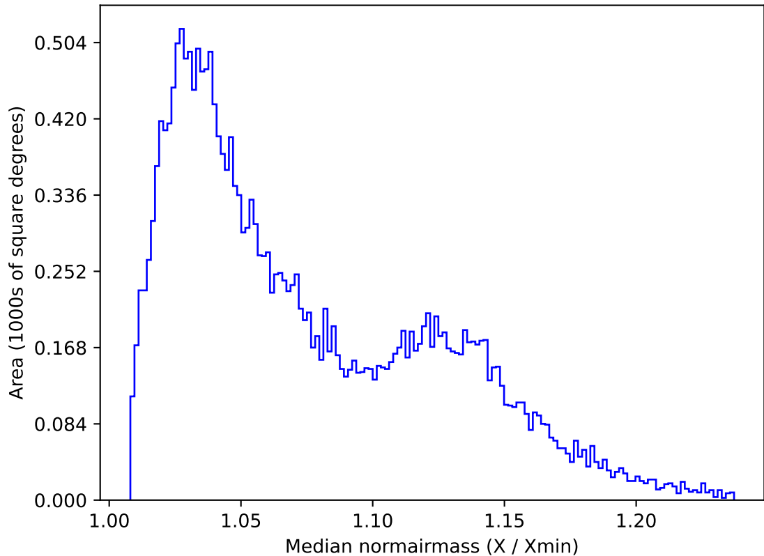
too_combined_s0.5_v3.4_10yrs All sky u band: Median normairmass
