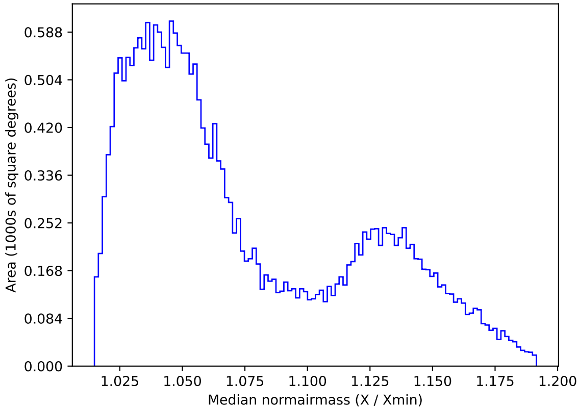
too_combined_s0.5_v3.4_10yrs All sky r band: Median normairmass
