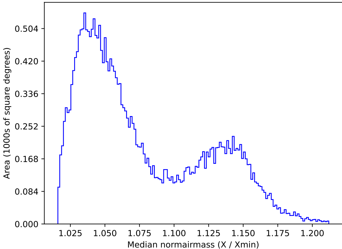
too_combined_s0.5_v3.4_10yrs All sky i band: Median normairmass
