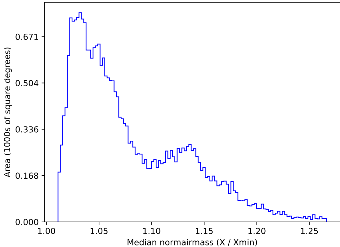
too_combined_s0.5_v3.4_10yrs All sky g band: Median normairmass
