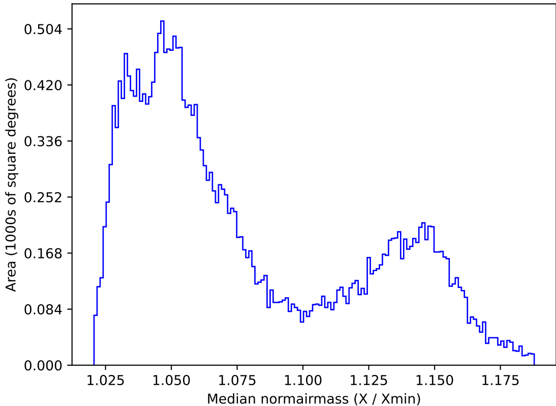
too_combined_s0.5_v3.4_10yrs All sky all bands: Median normairmass
