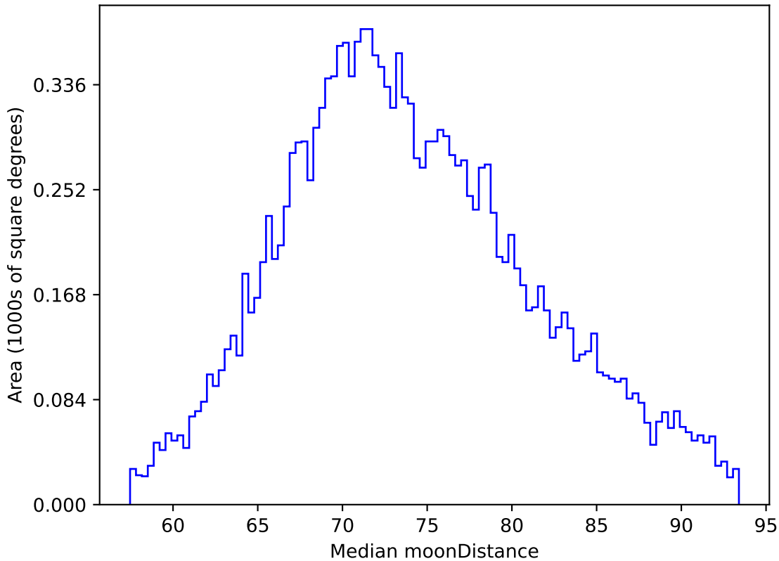
too_combined_s0.5_v3.4_10yrs WFD z band: Median moonDistance
