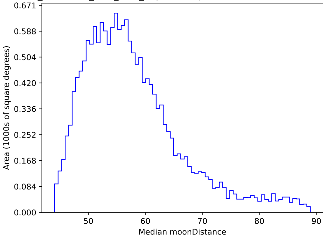
too_combined_s0.5_v3.4_10yrs WFD y band: Median moonDistance
