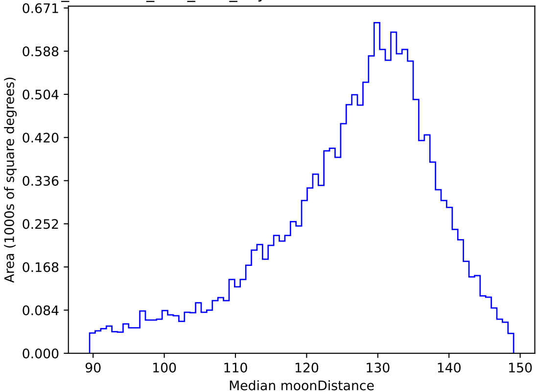
too_combined_s0.5_v3.4_10yrs WFD u band: Median moonDistance
