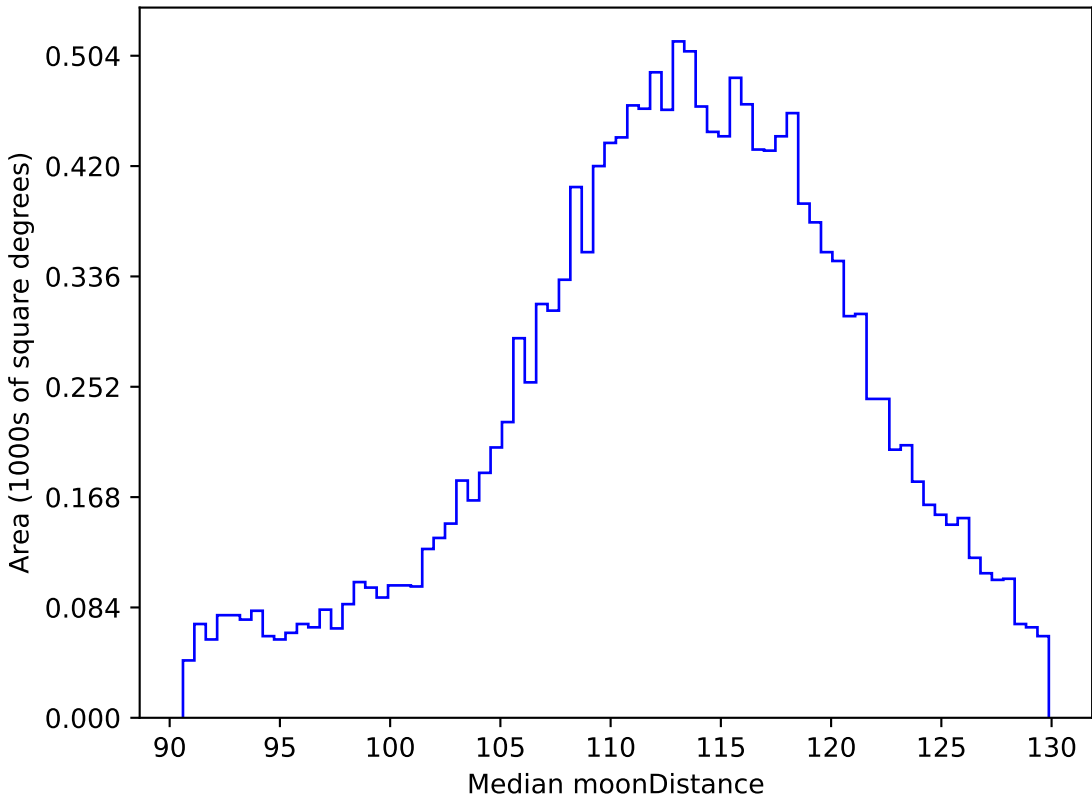
too_combined_s0.5_v3.4_10yrs WFD r band: Median moonDistance
