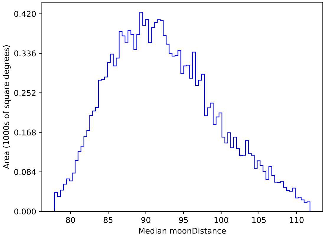
too_combined_s0.5_v3.4_10yrs WFD i band: Median moonDistance
