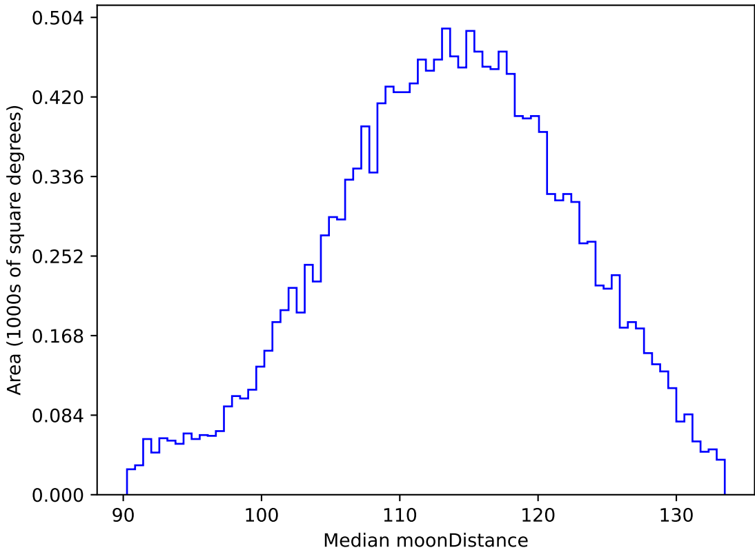
too_combined_s0.5_v3.4_10yrs WFD g band: Median moonDistance
