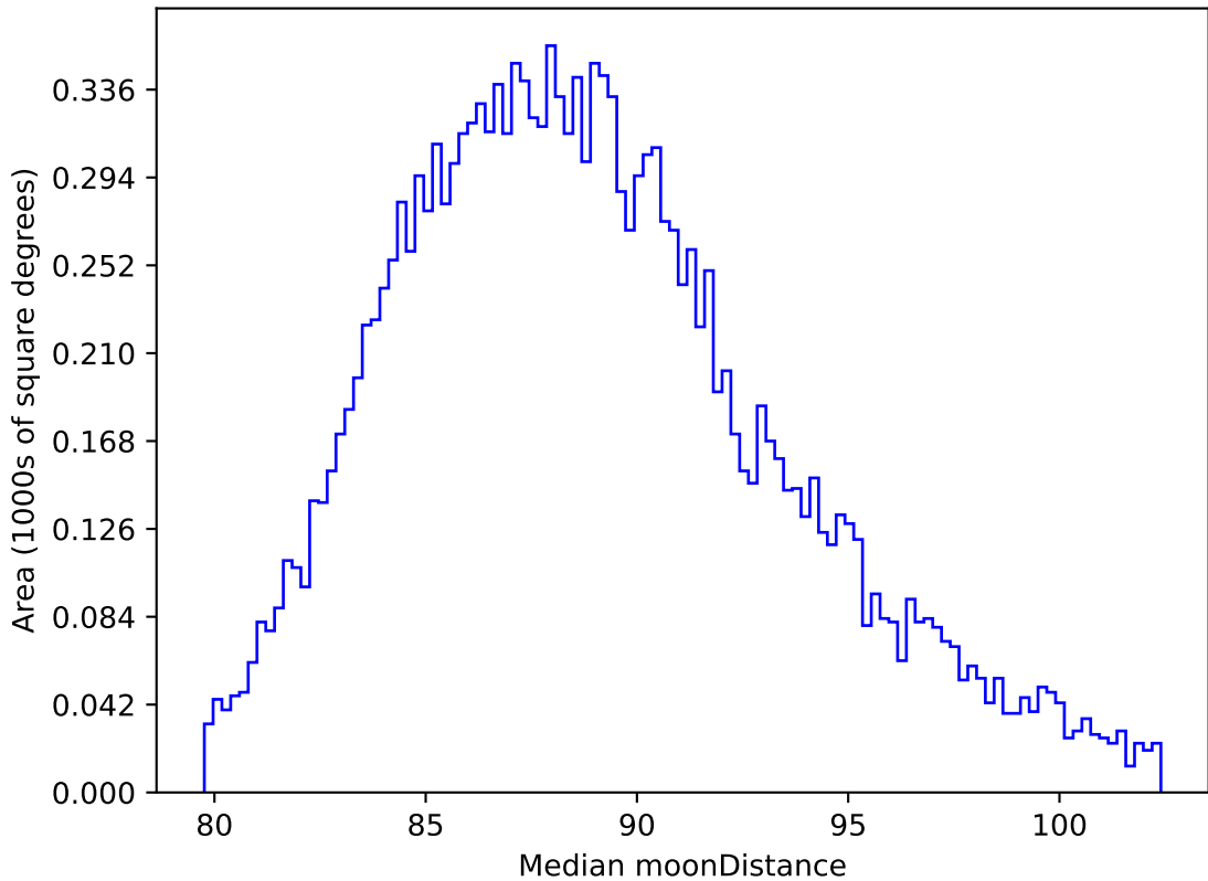
too_combined_s0.5_v3.4_10yrs WFD all bands: Median moonDistance
