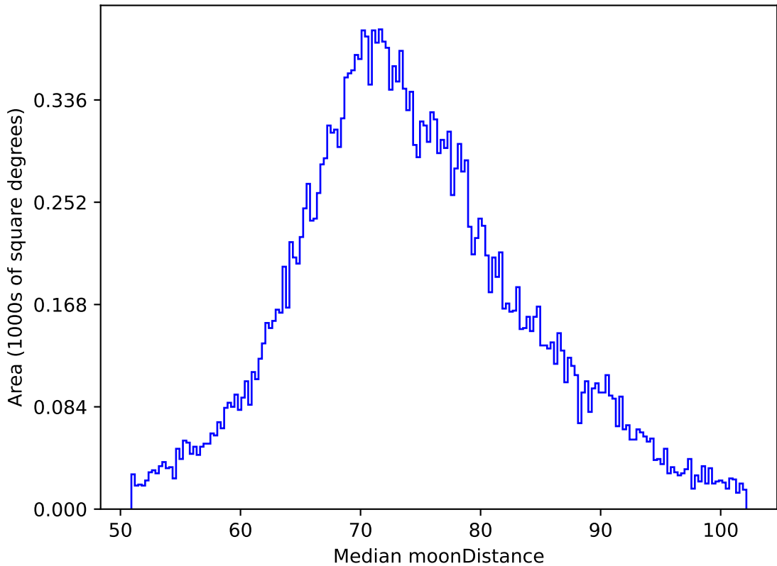
too_combined_s0.5_v3.4_10yrs All sky z band: Median moonDistance
