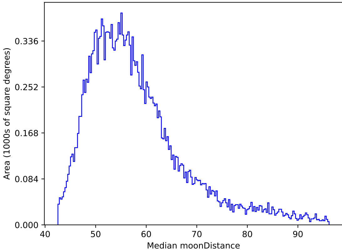
too_combined_s0.5_v3.4_10yrs All sky y band: Median moonDistance
