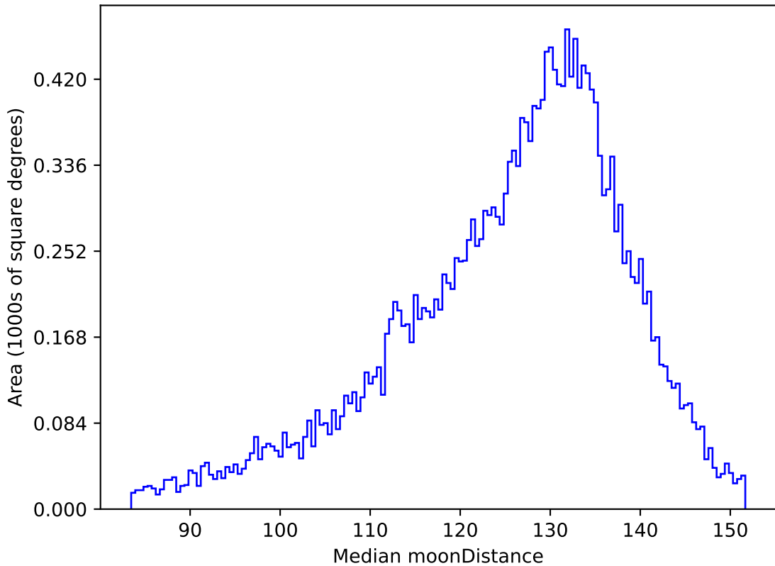
too_combined_s0.5_v3.4_10yrs All sky u band: Median moonDistance
