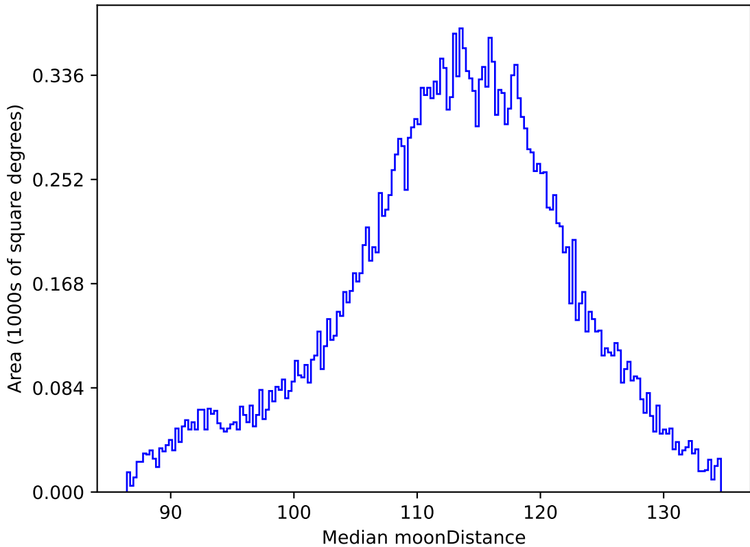
too_combined_s0.5_v3.4_10yrs All sky r band: Median moonDistance
