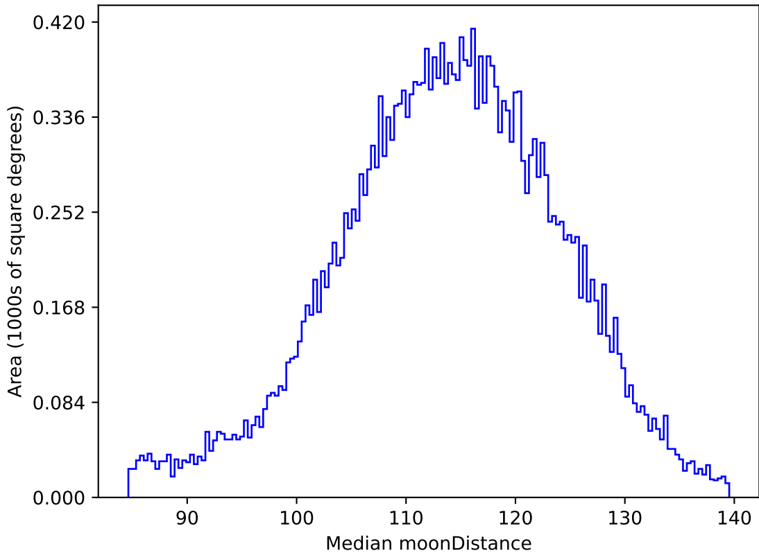
too_combined_s0.5_v3.4_10yrs All sky g band: Median moonDistance
