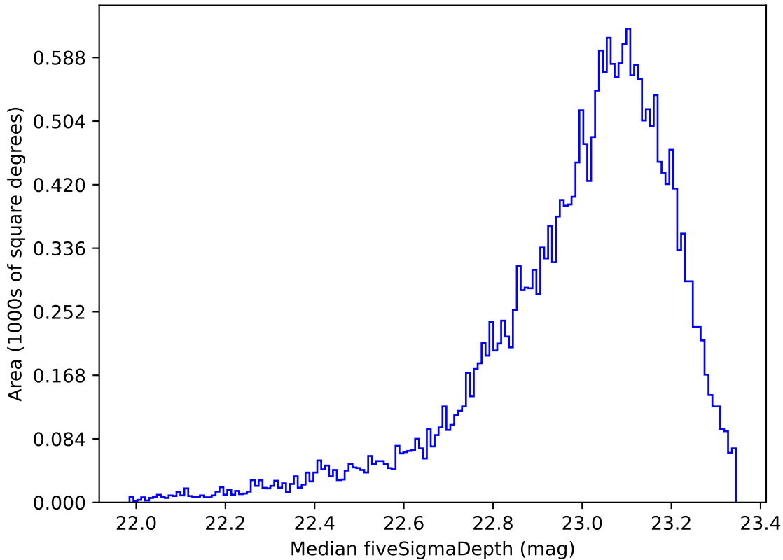
too_combined_s0.5_v3.4_10yrs Yr 1 z band: Median fiveSigmaDepth
