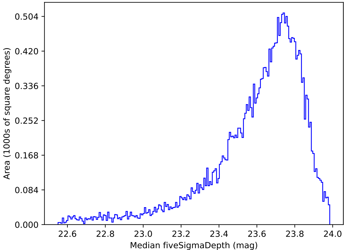
too_combined_s0.5_v3.4_10yrs Yr 1 i band: Median fiveSigmaDepth
