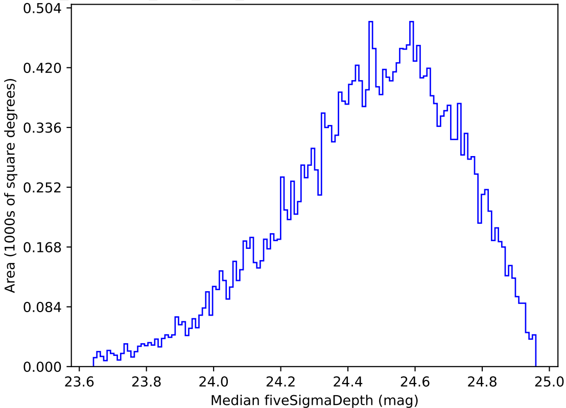
too_combined_s0.5_v3.4_10yrs Yr 1 g band: Median fiveSigmaDepth
