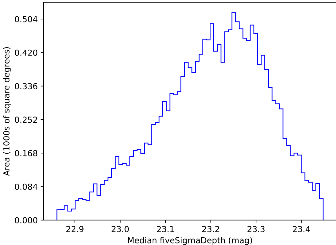
too_combined_s0.5_v3.4_10yrs WFD u band: Median fiveSigmaDepth
