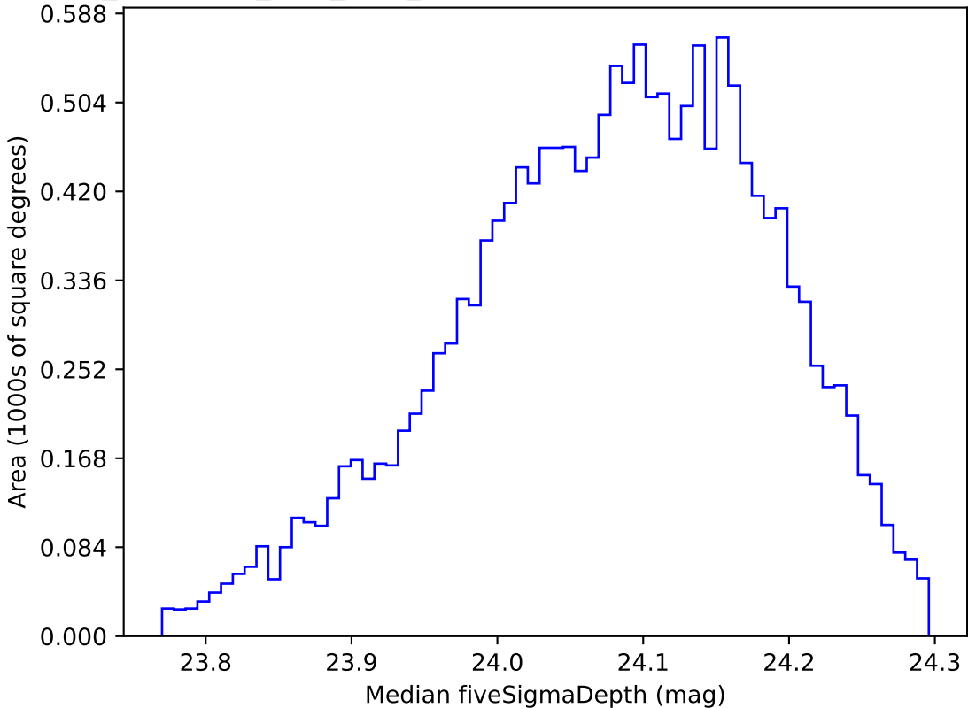
too_combined_s0.5_v3.4_10yrs WFD r band: Median fiveSigmaDepth
