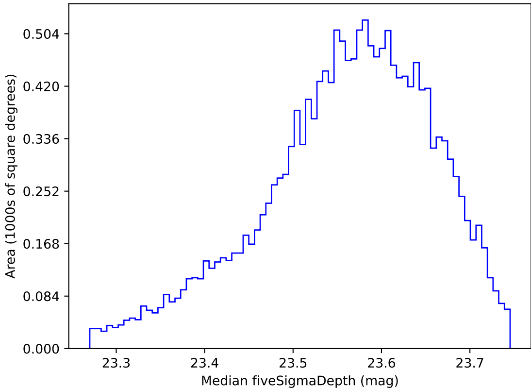
too_combined_s0.5_v3.4_10yrs WFD i band: Median fiveSigmaDepth
