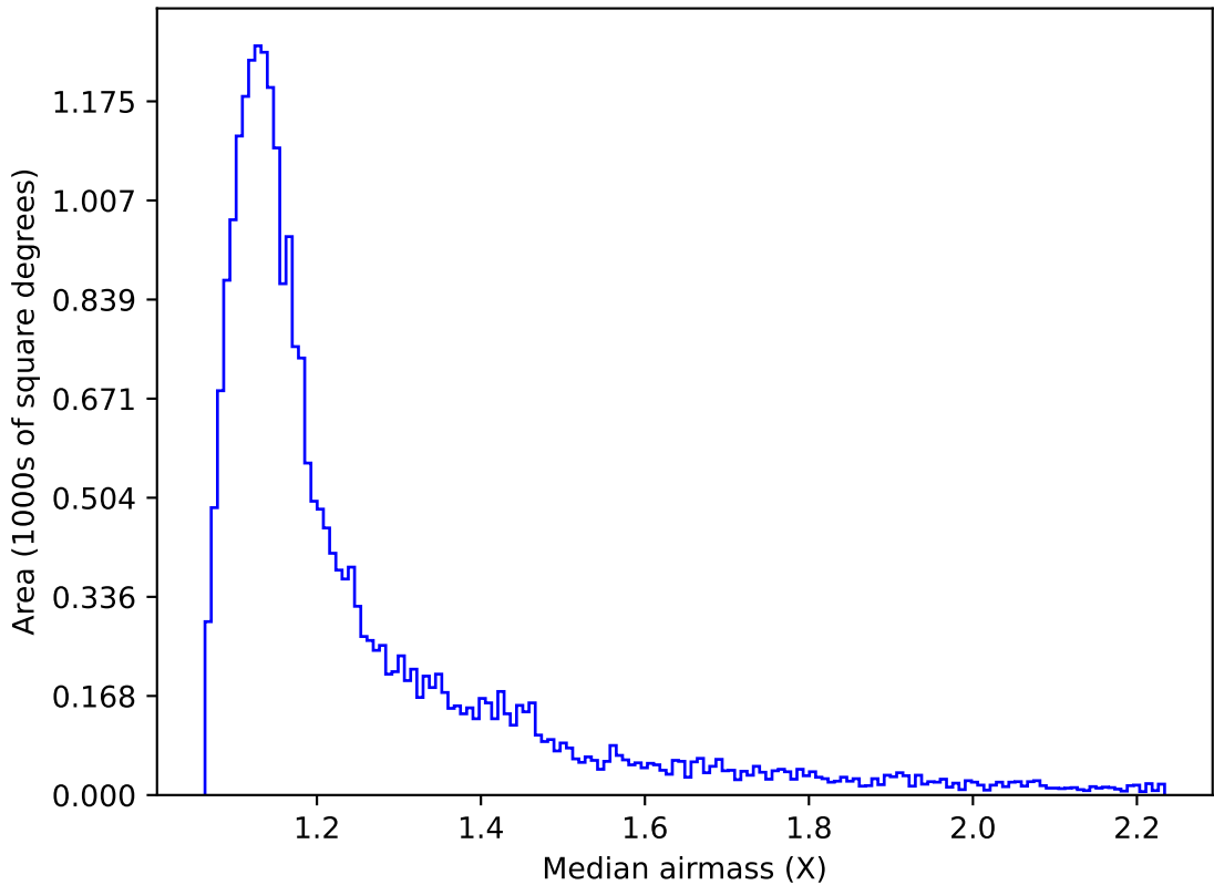
too_combined_s0.5_v3.4_10yrs Yr 1 z band: Median airmass
