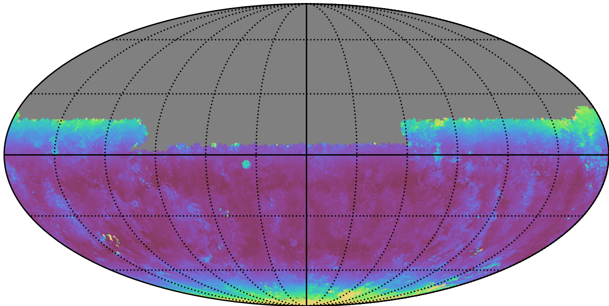
too_combined_s0.5_v3.4_10yrs Yr 1 y band: Median airmass
