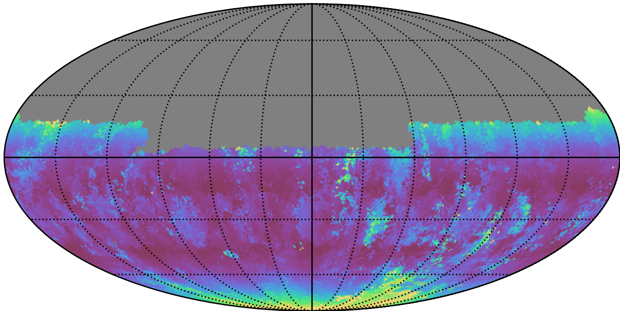
too_combined_s0.5_v3.4_10yrs Yr 1 u band: Median airmass
