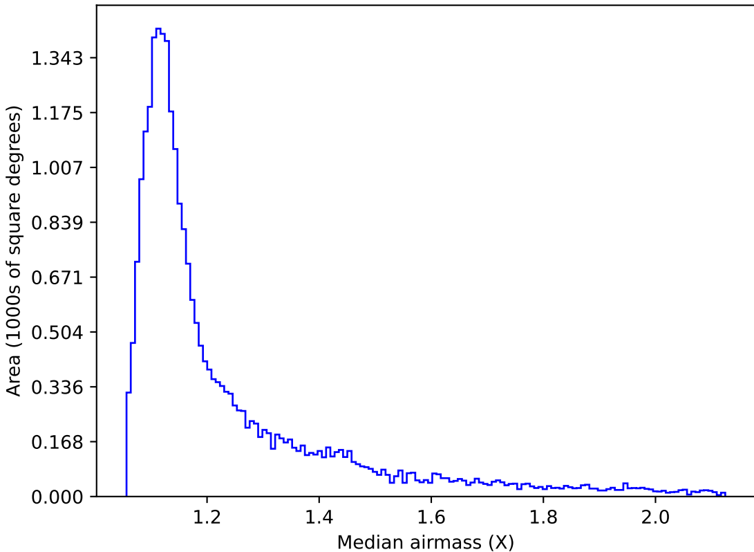
too_combined_s0.5_v3.4_10yrs Yr 1 i band: Median airmass
