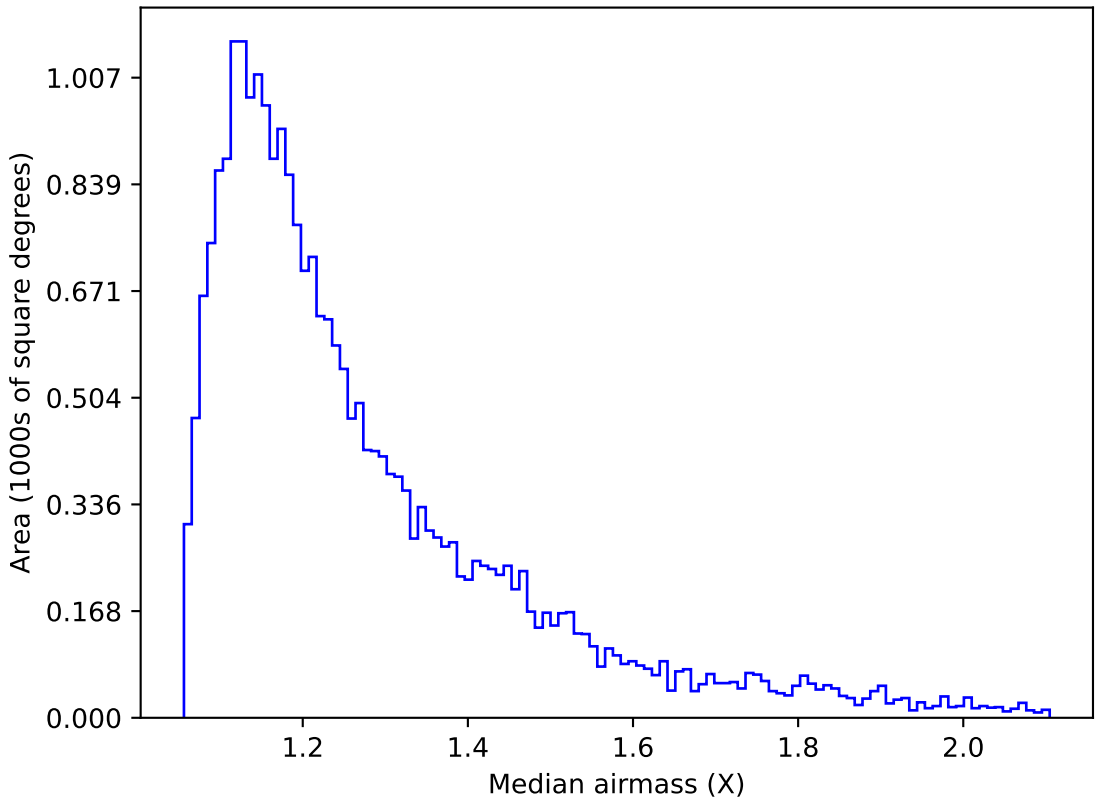
too_combined_s0.5_v3.4_10yrs Yr 1 g band: Median airmass
