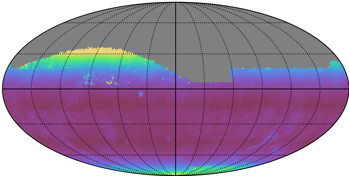
too_combined_s0.5_v3.4_10yrs Yr 1 all bands: Median airmass
