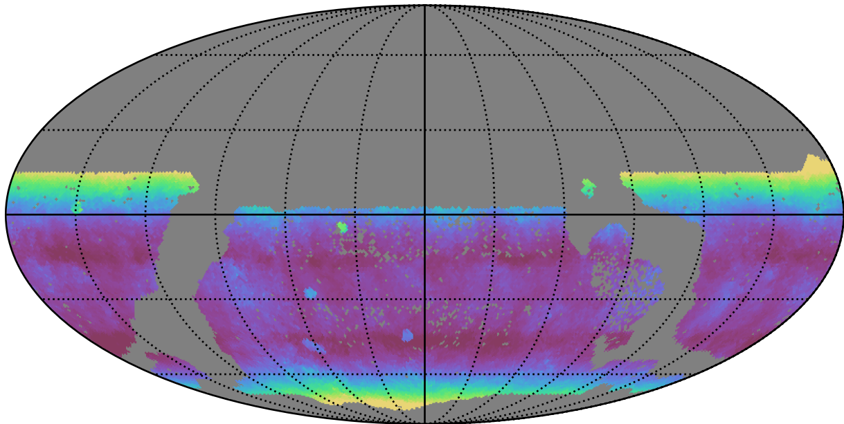
too_combined_s0.5_v3.4_10yrs WFD y band: Median airmass
