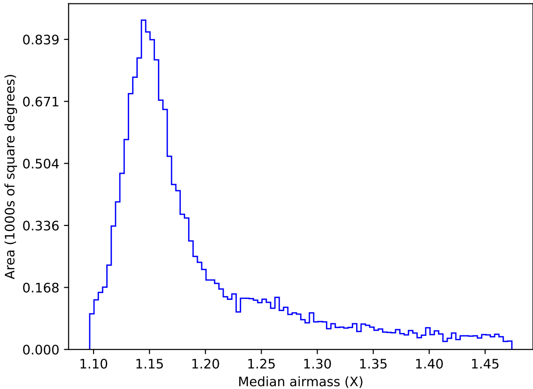
too_combined_s0.5_v3.4_10yrs WFD y band: Median airmass
