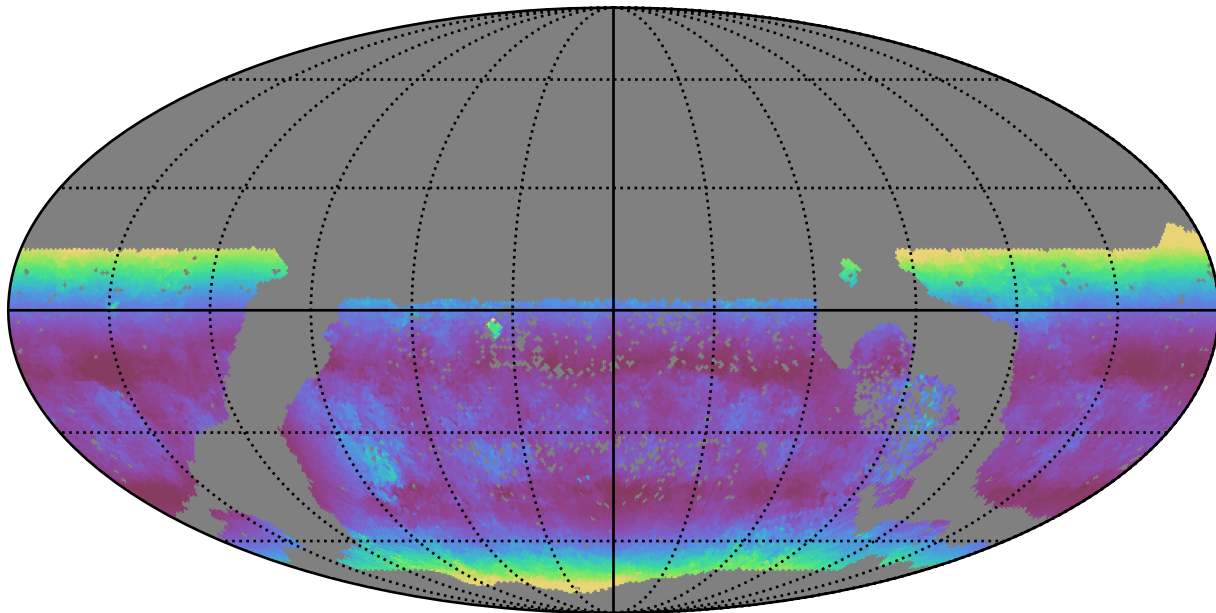
too_combined_s0.5_v3.4_10yrs WFD u band: Median airmass
