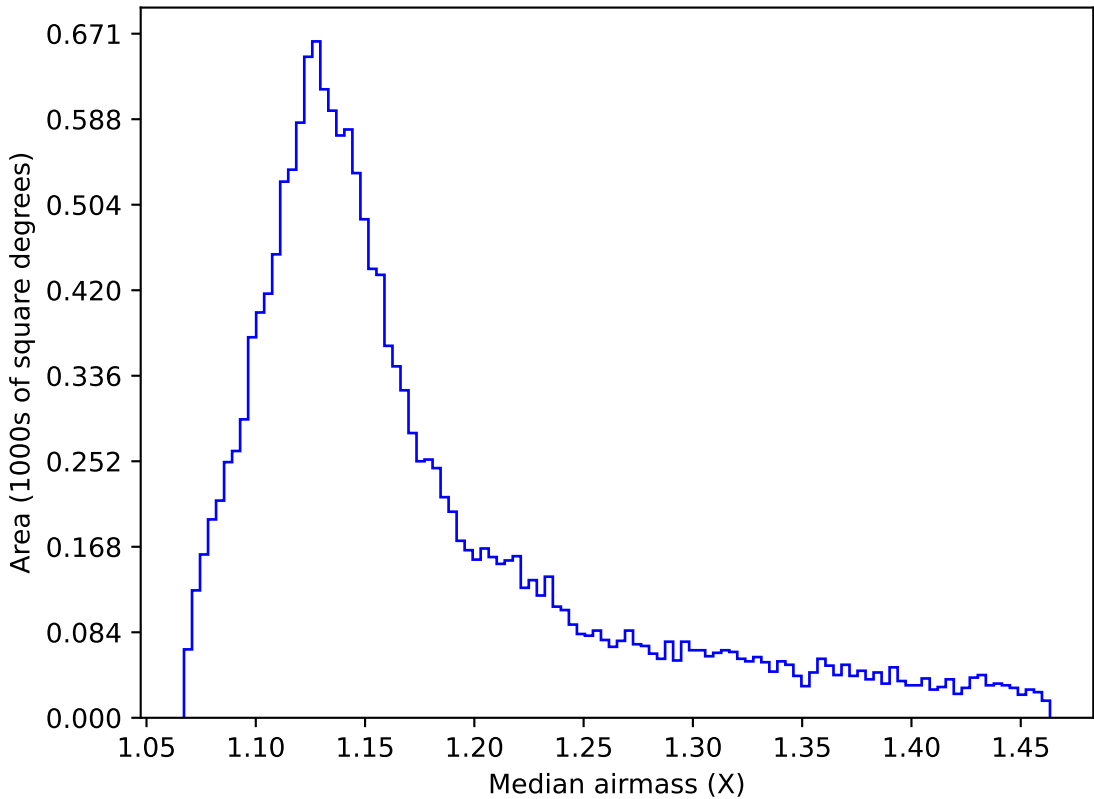
too_combined_s0.5_v3.4_10yrs WFD u band: Median airmass
