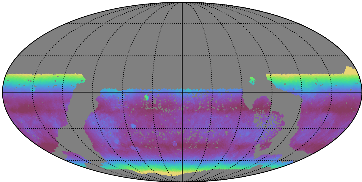
too_combined_s0.5_v3.4_10yrs WFD r band: Median airmass
