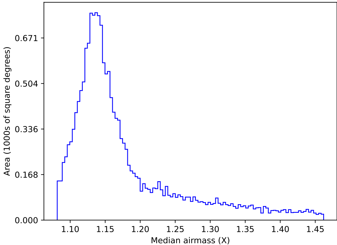
too_combined_s0.5_v3.4_10yrs WFD r band: Median airmass
