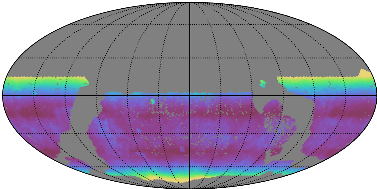
too_combined_s0.5_v3.4_10yrs WFD i band: Median airmass
