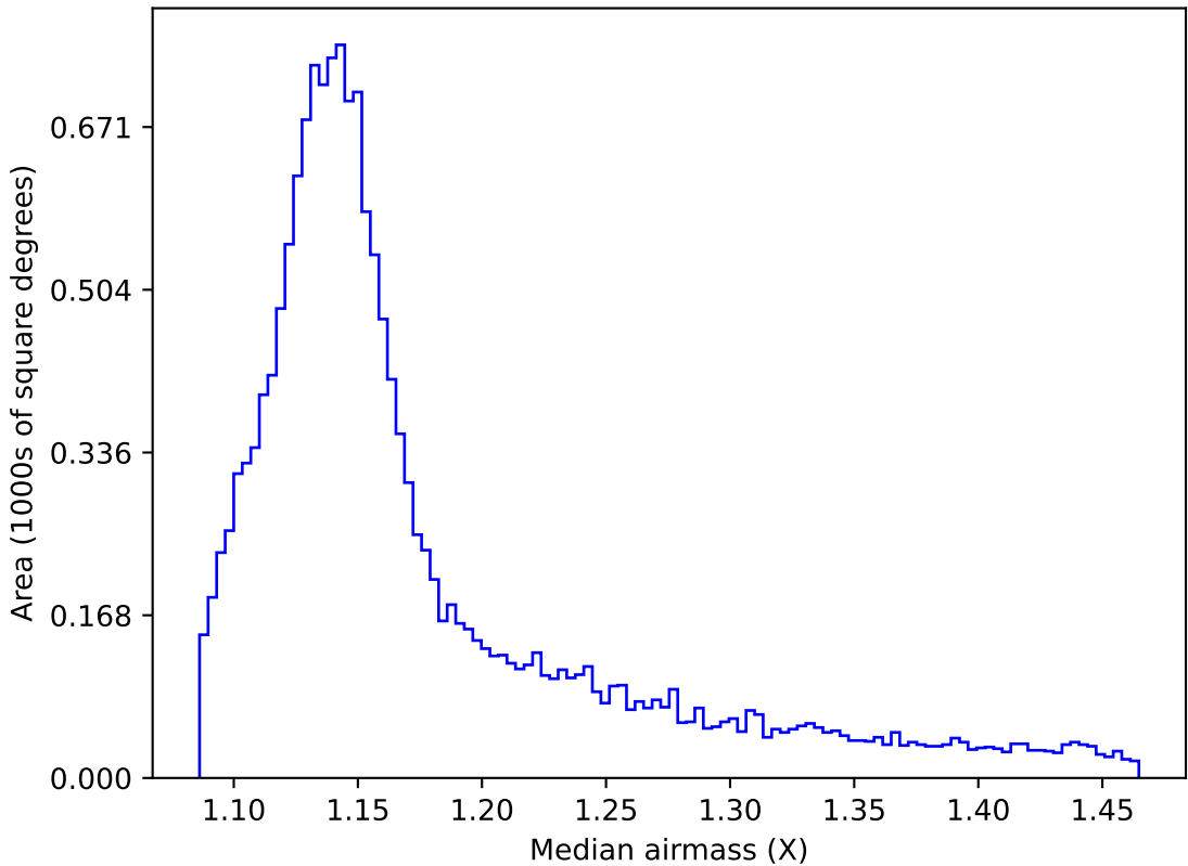
too_combined_s0.5_v3.4_10yrs WFD i band: Median airmass
