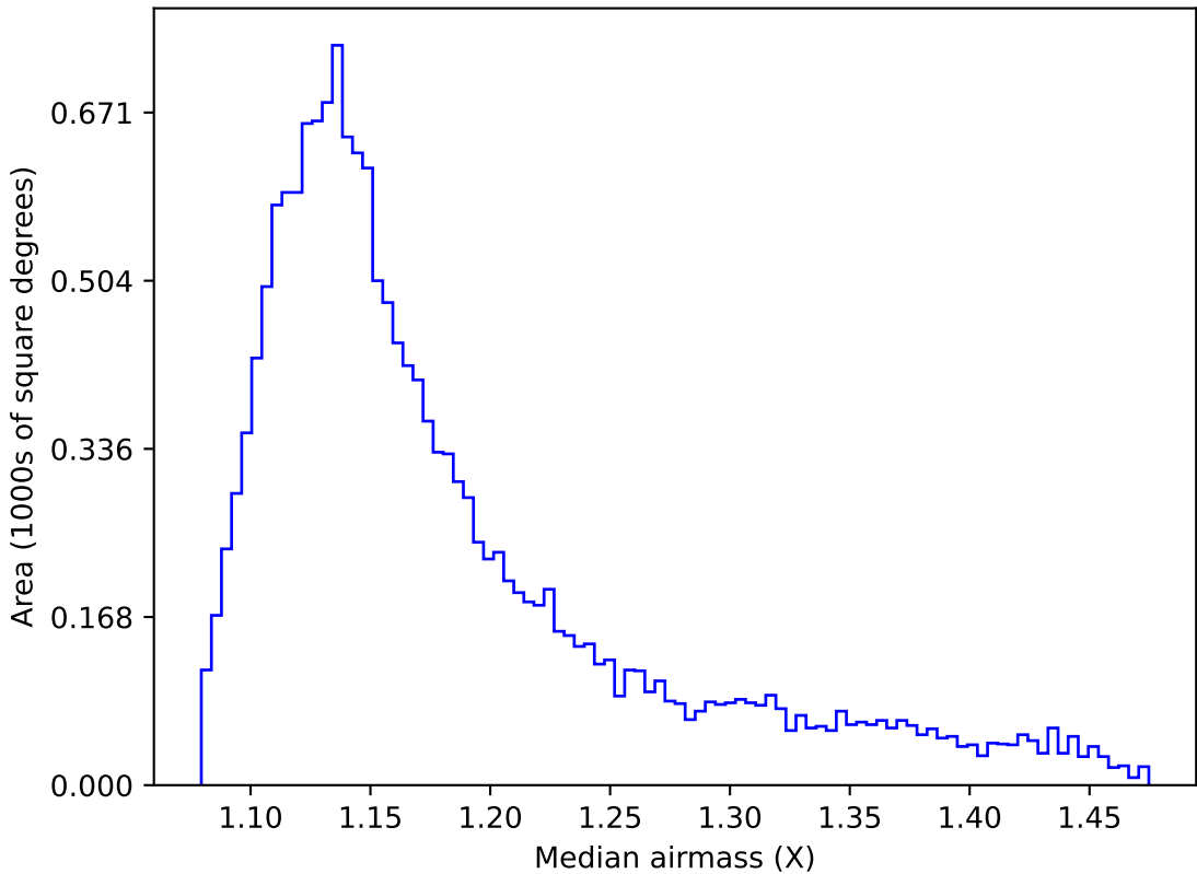
too_combined_s0.5_v3.4_10yrs WFD g band: Median airmass
