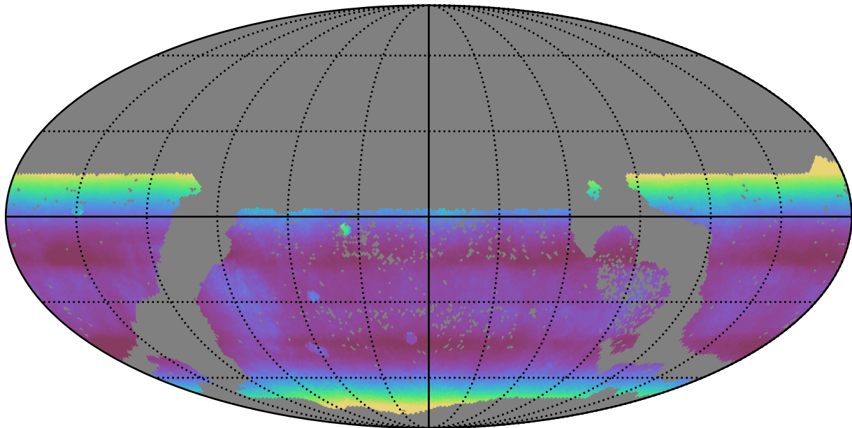
too_combined_s0.5_v3.4_10yrs WFD all bands: Median airmass
