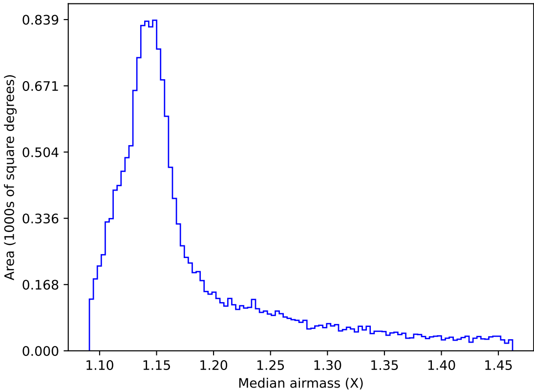
too_combined_s0.5_v3.4_10yrs WFD all bands: Median airmass
