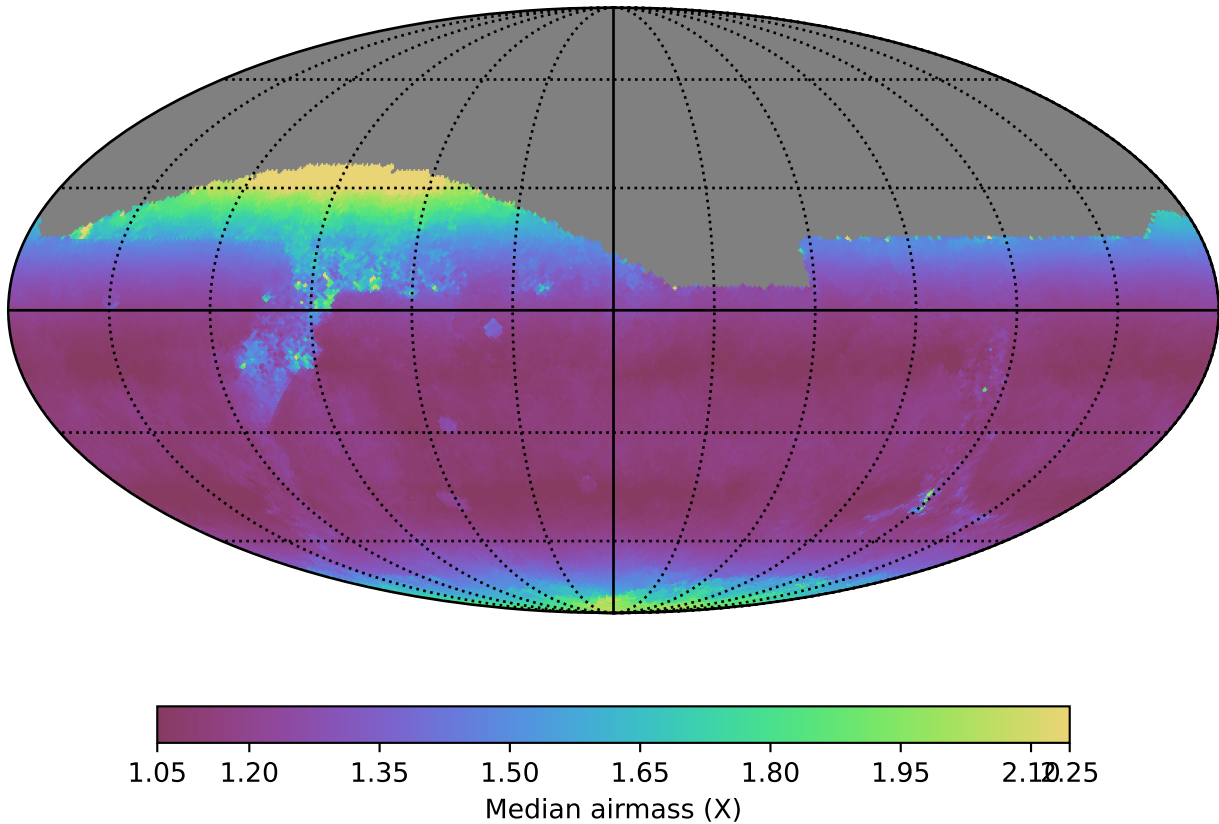
too_combined_s0.5_v3.4_10yrs All sky z band: Median airmass
