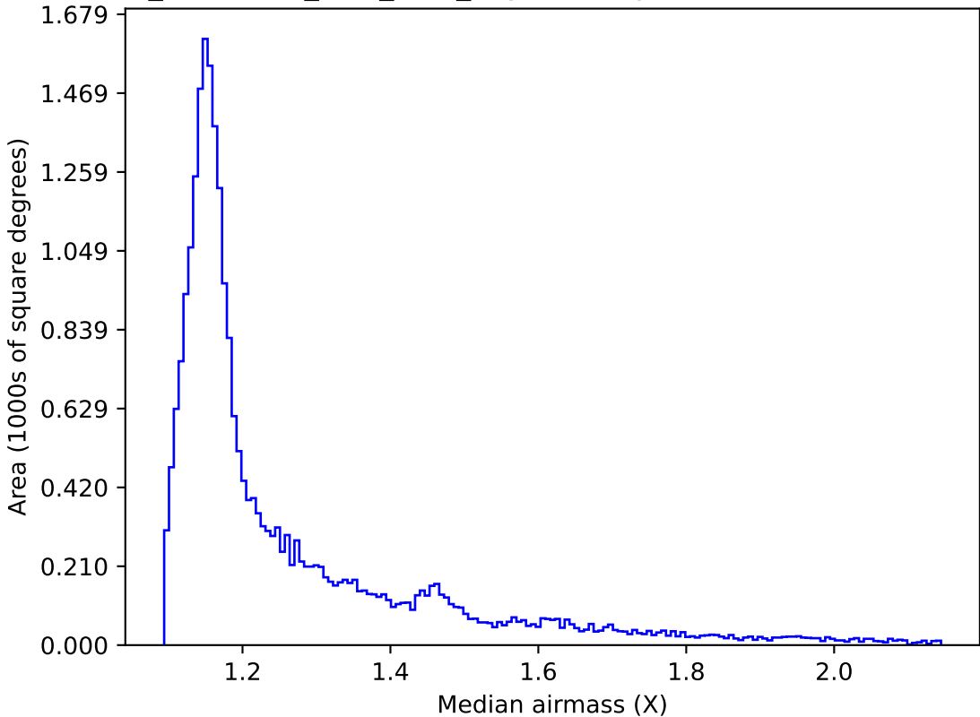
too_combined_s0.5_v3.4_10yrs All sky z band: Median airmass
