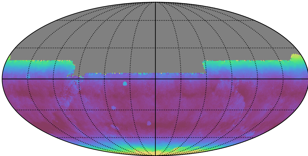
too_combined_s0.5_v3.4_10yrs All sky y band: Median airmass
