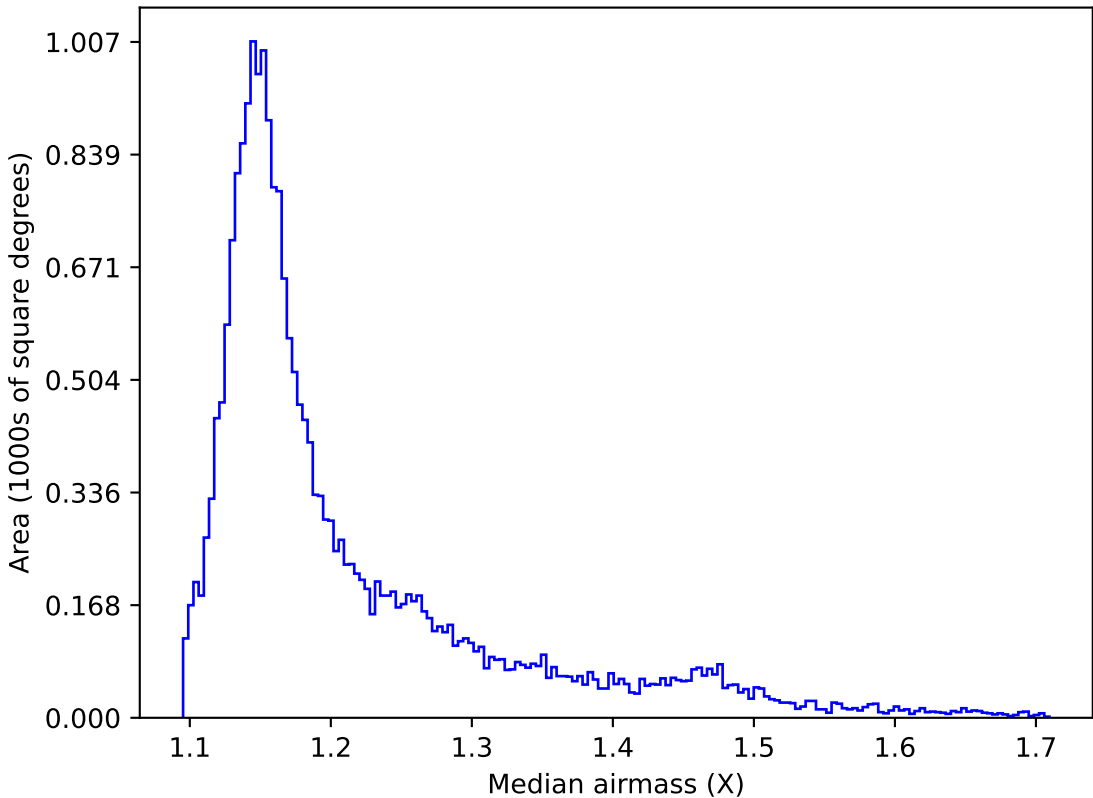
too_combined_s0.5_v3.4_10yrs All sky y band: Median airmass
