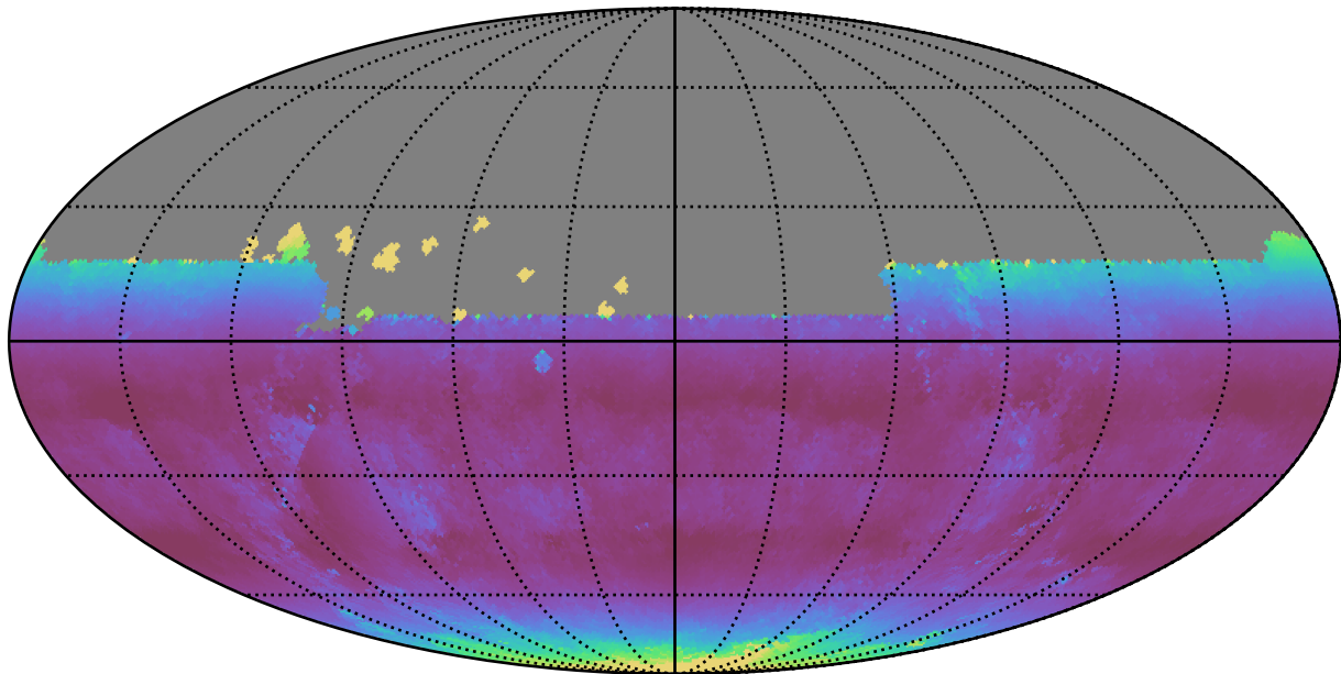
too_combined_s0.5_v3.4_10yrs All sky u band: Median airmass
