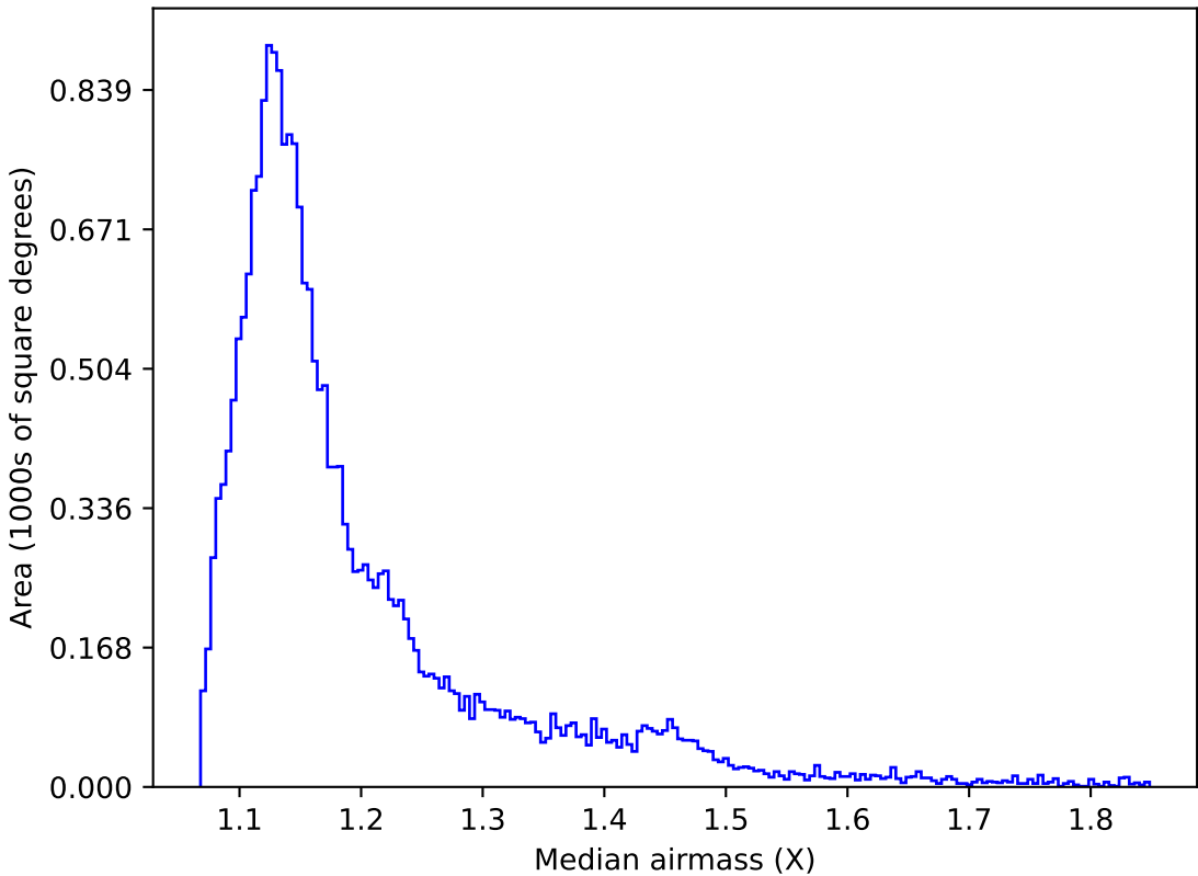
too_combined_s0.5_v3.4_10yrs All sky u band: Median airmass
